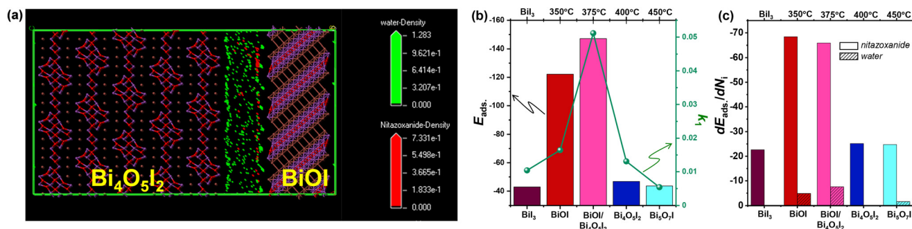
Fig. 9 (a) Visualization of adsorption of nitazoxanide and water molecules onto the BiOI/Bi 4 O 5 I 2 interface. The red, violet, and brown spheres represent oxygens, bismuth, and iodine. Isosurface field density: green is water and red is nitazoxanide. (b) Effect of adsorption energy on degradation constants for different bismuth (oxy)iodide phases. (c) Differential adsorption energy of nitazoxanide and water molecules on different bismuth (oxy)iodide phases.
