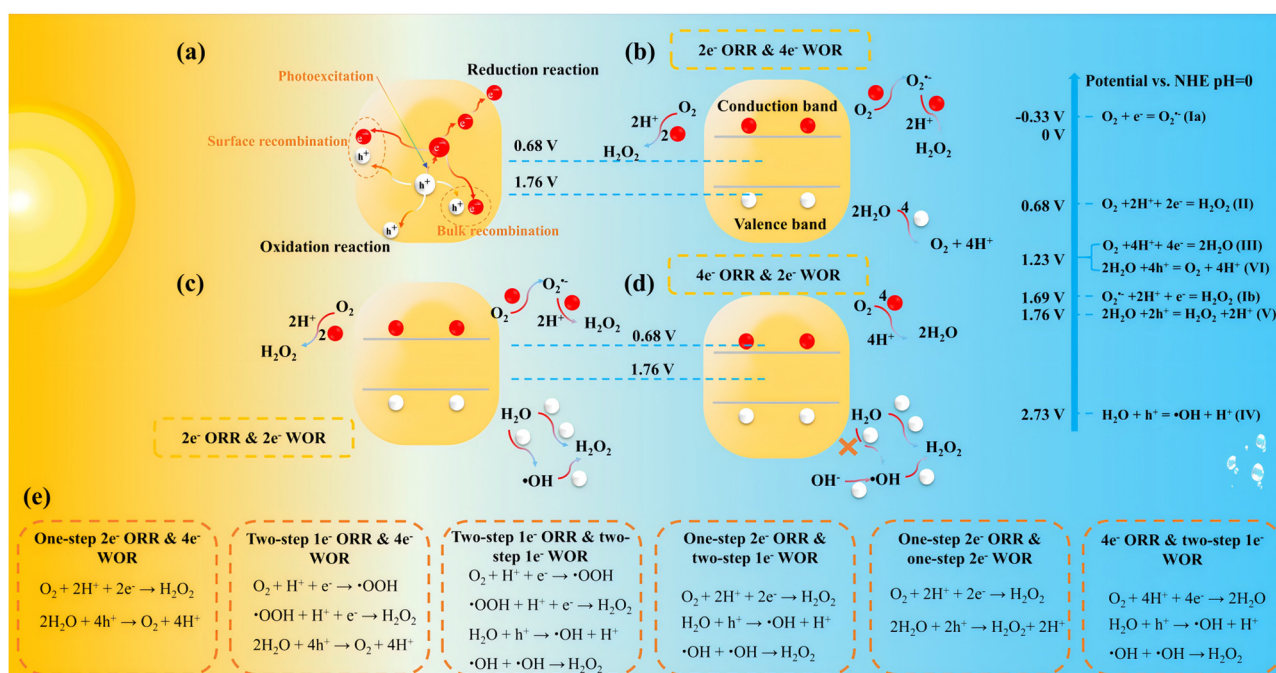
Fig. 2 (a) Photoexcitation and charge transfer pathways in a photocatalyst. The Scheme of \text{H}_2\text{O}_2 producing via (b) 2\text{e}^- ORR and 4\text{e}^- WOR pathway, (c) 2\text{e}^- ORR and 2\text{e}^- WOR pathway and (d) 4\text{e}^- ORR and 2\text{e}^- WOR pathway. (e) Classical combinations of ORR and WOR pathways.
