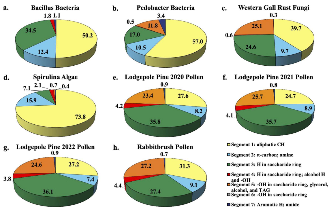
Fig. 1 Pie chart percent distribution of functional groups in select bioaerosol extracts (water extracts resuspended in \text{DMSO}-d_6 ), analyzed with ^1\text{H} -NMR spectroscopy. Each pie slice corresponds to chemical shift segments 1 through 7 (see legend). Details on each segment can be found in Table 2.
