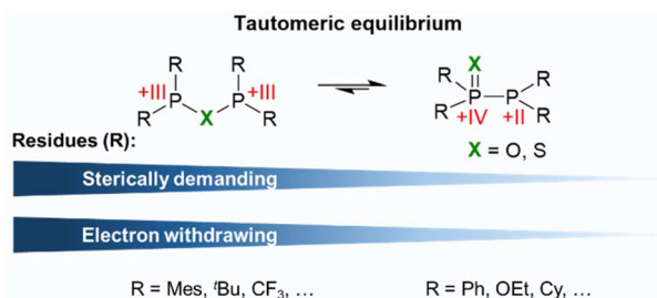
Fig. 2 Phosphotropic tautomerism of the PXP/PPX ligand with the oxidation states of the phosphorus atoms given in red. With sterically more demanding or electron withdrawing substituents on the phosphorus atoms, the PXP-based tautomer is favoured, whereas in the case of sterically less demanding or less electron withdrawing groups the PPX tautomer dominates.
