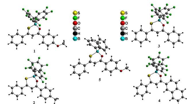
Fig. 1 X-ray crystal structure of complexes 1–5 with ball and stick model (diamond view).
