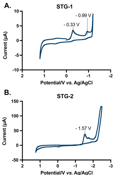
Fig. 3 Cyclic voltammograms of STG compounds (5 mM) in DMSO with [\text{N}(\text{Bu})_4\text{PF}_6] as supporting electrolyte. Potentials are shown vs. Ag/AgCl. (A) Voltammogram of STG-1 showing two reduction events at -0.33 V and -0.99 V. (B) Voltammogram of STG-2 showing one reduction event at -1.57 V. Data collected with a glassy carbon working electrode and Pt counter electrode.
