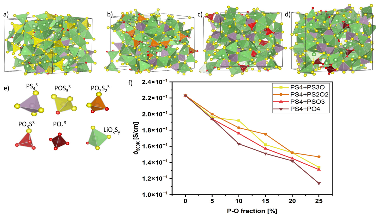
Fig. 8 (a–d) Simulated structures with only \text{PS}_4 and \text{PS}_3\text{O} (a), \text{PO}_2\text{S}_2 (b), \text{PO}_3\text{S} (c), \text{PO}_4 (d) units at 20% P–O fraction. (e) Description of the different polyhedra. (f) Calculated Li-ion conductivities against P–O fraction for the displayed structures.
