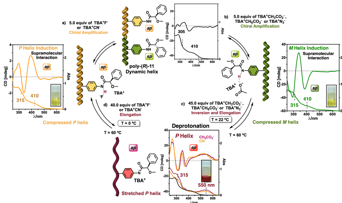
Fig. 23 (a) P and (b) M helix induction in poly-( R )- 11 by addition of 5.0 equiv. of TBAA (A = fluoride or cyanide) or (A = acetate, benzoate or azide) respectively. Elongation and P helix induction in poly-( R )- 11 by addition of (c) 45.0 equiv. of TBAA (A = acetate, benzoate or azide) at rt or (d) 40.0 equiv. of TBAA (A = fluoride or cyanide) at 0 °C. Reproduced from ref. 189 with permission from Elsevier, copyright 2021.
