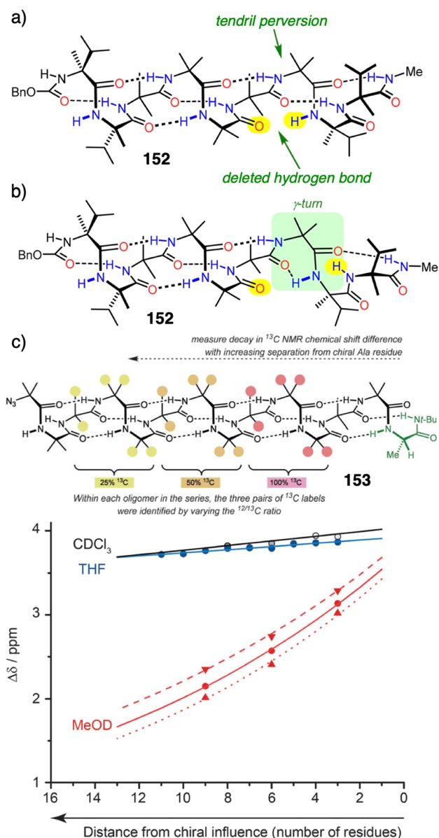
Fig. 74 (a) Tendrils or perversions and (b) \gamma -turn in AIB foldamer 152. (c) Chemical shift differences ( \Delta\delta ) measured in a series of three 'frame-shifted' oligomers, each containing three pairs of abundance-labelled (100%, 50% or 25%) ^{13}\text{C} labels. Screw-sense preference exhibited by Aib oligomer 153 decays as a terminal chiral influence becomes more distant. Reproduced from ref. 358 with permission from the Royal Society of Chemistry, copyright 2016.
