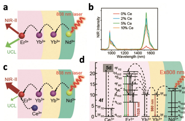
Fig. 14 (a) Schematic illustration of the energy transfer path from Nd 3+ to inner Er 3+ for luminescence without (a) and with (c) Ce 3+ -ion doping. (b) The downconverting NIR fluorescence spectra of NaYbF 4 :2% Er, y% Ce@NaYF 4 :10% Yb@NaYF 4 :50% Nd (y = 0, 2, 5, and 10). (d) Detailed illustration of the energy transfer from Nd 3+ to Er 3+ , emitting NIR-II luminescence at 1525 nm under 808 nm excitation. Reproduced with permission from ref. 138. Copyright 2020, Royal Society of Chemistry.
