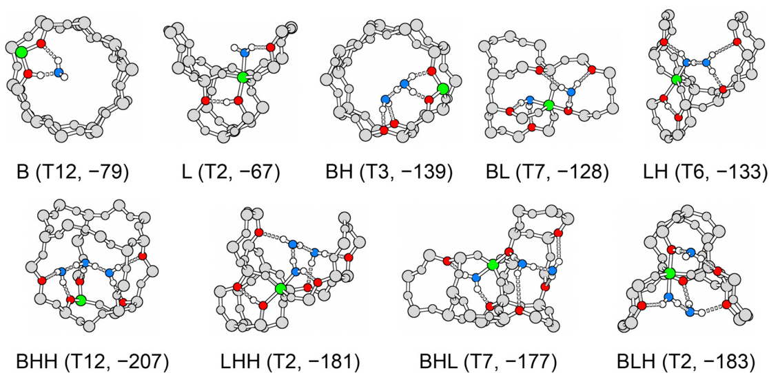
Fig. 9 Most stable adsorption structures for each interaction motif. Framework position and MP2+ \Delta\text{ACC} adsorption energies in \text{kJ mol}^{-1} in parenthesis. Colour code: aluminium – green, framework oxygen accepting hydrogen bond – red, oxygen in water molecules – blue, framework silicon and oxygen – grey, hydrogen – white.
