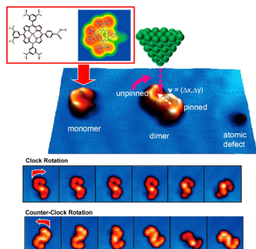
Fig. 11 A supramolecularly recombinable molecular rotor of Pt-porphyrin supramolecular dimer supported on an Au(111) surface with rotation behaviors in a highly directional manner, where the direction of rotation of this molecular rotor is determined solely by the surface chirality of the dimer. Reprinted with permission from ref. 75. Copyright 2015 American Chemical Society.
