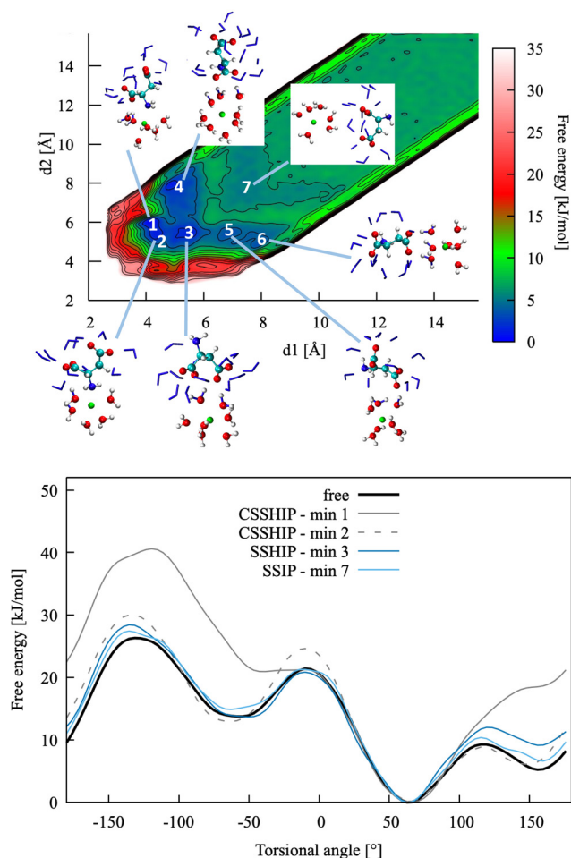
Fig. 6 Top: Pairing free energy of \text{Ca}^{2+} L-Asp ^{2-} projected along two Ca–C distances, d1 and d2 (defined in Fig. 5). Minima correspond to contact (N–Ca) plus solvent-shared (C–Ca) ion pairs (CSSHIP, 1 and 2), solvent-shared ion pairs (SSHIP, 3 to 6) and solvent separated ion pairs (SSIP, 7). Examples of configurations for each minimum are provided, with atoms coloured as in Fig. 4. Bottom: Rotational free energy profile around the -\beta torsional angle of L-Asp ^{2-} , free and bound with \text{Ca}^{2+} .
