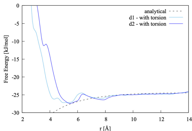
Fig. 7 Pairing free energy of \text{Ca}^{2+} L-Asp ^{2-} projected along two Ca–C distance and obtained with sampling along the -\beta torsional angle collective variable.
