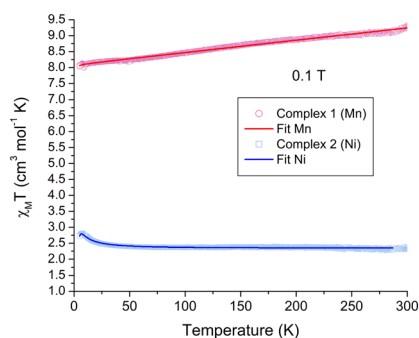
Fig. 5 \chi_M T vs. T magnetic behavior for complexes 1 and 2 . The solid lines represent the best fit for both complexes.
