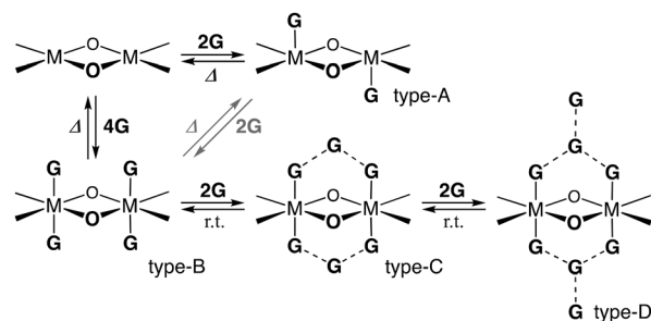
Scheme 2 Four-types of the guest inserted structures of dinuclear metal complexes (M = Ni 2+ or Cu 2+ ).
