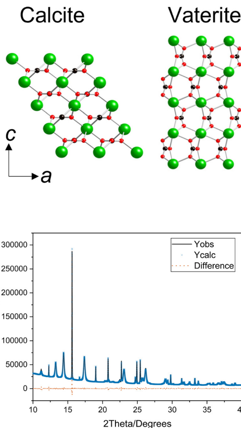
Fig. 2 (a) Crystal structures of calcite (left) and vaterite (right), where green is calcium, black is carbon and red is oxygen. Both crystal structures are orientated in the same direction to highlight the difference between the a and c lattice parameters. The vaterite structure shown is a simplified version of the Kamhi structure, 33 removing the disorder to facilitate comparison. (b) Diffraction pattern for sample 68-08 with the observed and calculated data and the difference.
