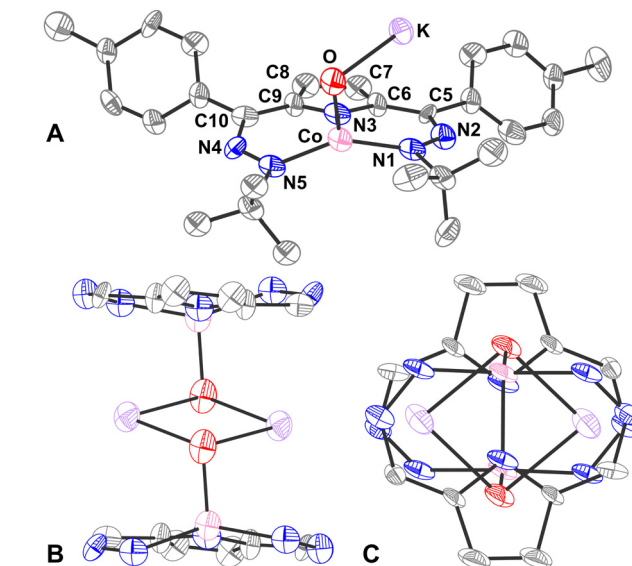
Fig. 1 (A) SXRD structure of 1 . (A) One half of the dimeric unit with the full DHP ligand. (B) A side view focusing on the O 2 K 2 core with peripheral groups omitted. (C) A top view showing the stacked interactions with the K cations with peripheral groups omitted. Co (pink), N (blue), C (grey), O (red), K (violet). Ellipsoids at 50% and hydrogens omitted for clarity.
