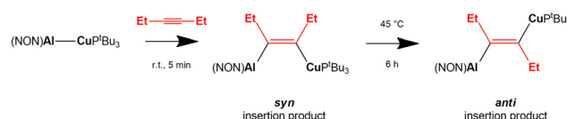
Scheme 8 Experimental insertion of internal 3-hexyne in the Cu–Al bond of the [\text{tBu}_3\text{PCuAl(NON)}] complex. 68
