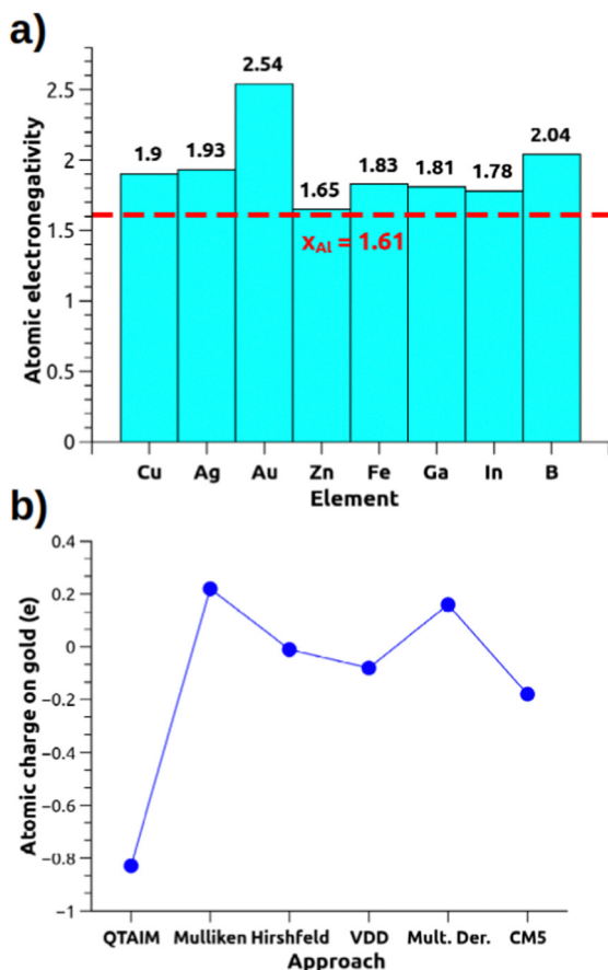
Fig. 3 (a) Pauling electronegativities for relevant elements of the periodic table. (b) Atomic charge on the Au atom for the [Bu_3PAuAl(NON)] complex calculated with different approaches (data taken from ref. 30).
