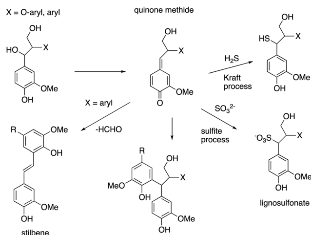
Fig. 10 Structures of condensed units found in Kraft lignin and lignosulfonate, formed from \beta -aryl ether units (X = O-aryl) and diarylpropane units (X = aryl).
