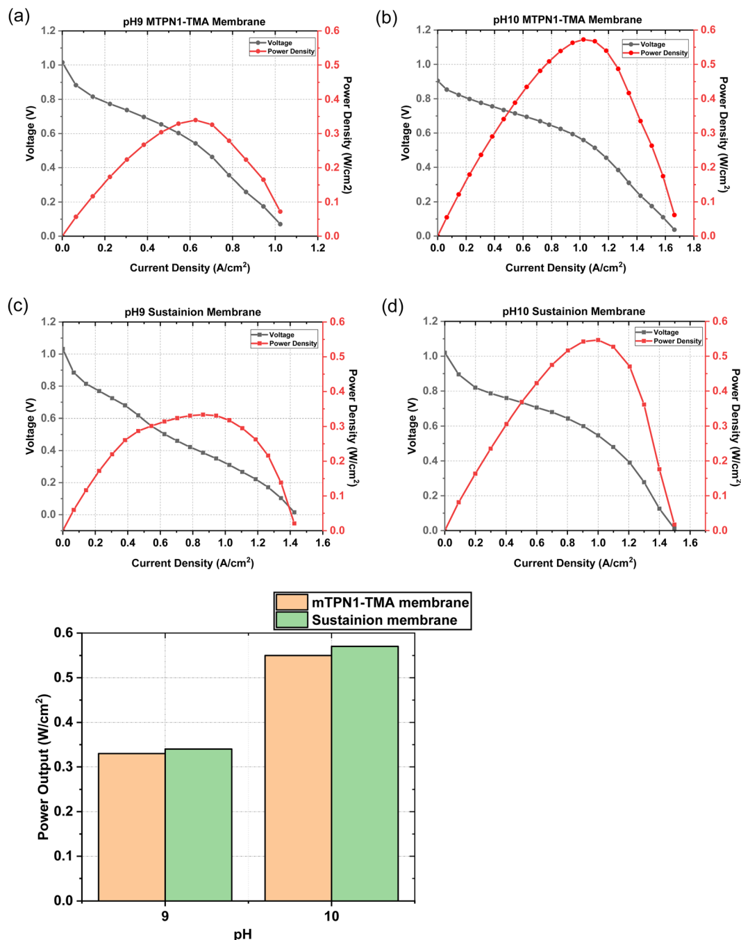
Fig. 8 Polarization Curves for (1) m TPN1-TMA membranes at (a) pH-9 (b) pH-10 and for (2) Sustainion membranes at (c) pH-9 (d) pH-10 (3) Power output vs. pH for m TPN1-TMA membranes and Sustainion membranes.
