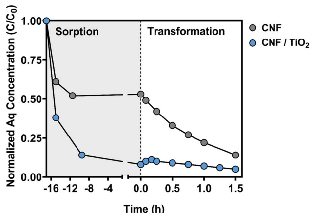
Fig. 5 Normalized aqueous (Aq) carbamazepine (CBZ) concentration ( C/C_0 ; C_0 = 10 \mu\text{M} CBZ) over time during the sorption and electrochemical (EC) transformation periods. CBZ sorption was conducted in the dark, without an applied potential. The EC transformation was conducted at +1.00 V (vs. Ag/AgCl). Data are shown for the optimal composite (0.45 g PAN/50 wt% \text{TiO}_2 /1000 °C) and for CNFs without \text{TiO}_2 carbonized at 1000 °C.
