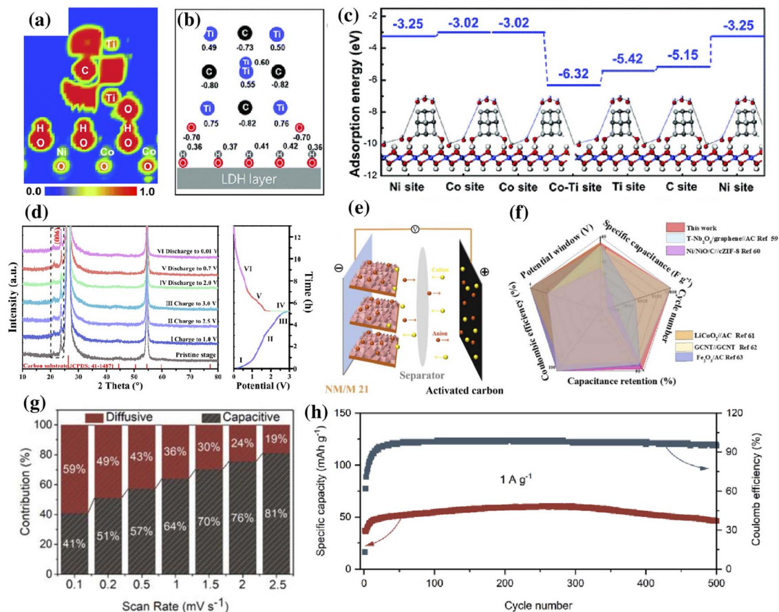
Fig. 5 (a) ELF mappings and (b) calculated charge of surface atoms of MQDs in Ni-Co LDH@MXene. (c) Calculated adsorption energies using hydroxide ( \text{OH}^- ) as an example for Ni-Co LDH@MXene (ref. 153). (d) Ex situ XRD patterns of NM/M 2:1/AC collected at various states, (e) schematic diagram of a NM/M 2:1/AC capacitor, and (f) comparison of its electrochemical performance with that of previously reported ASC devices. Reproduced with permission from ref. 154 copyright 2020, American Chemical Society. (g) Capacitive and diffusive contribution ratio of NiFe-LDH/MXene at respective scan rates. (h) Cycle stability of the NiFe-LDH/MXene//AC LIC at 1 \text{ A g}^{-1} . Reproduced with permission from ref. 152 copyright 2021, American Chemical Society.
