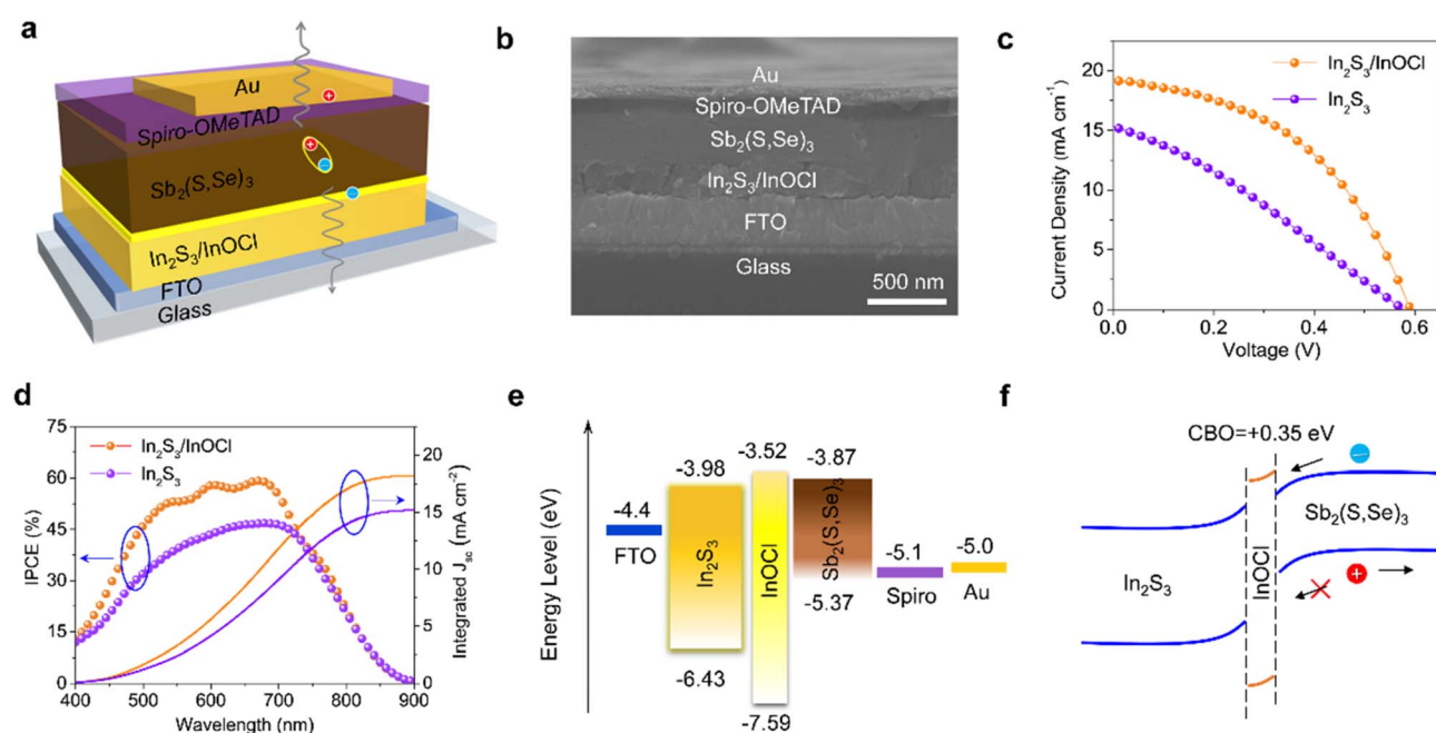
Fig. 4 (a and b) The schematic illustration and cross-sectional SEM image of a complete device with the configuration of FTO/ \text{In}_2\text{S}_3/\text{InOCl}/\text{Sb}_2(\text{S},\text{Se})_3/\text{spiro-OMeTAD}/\text{Au} , (c) J – V and (d) IPCE curves of the best-performing devices based on \text{In}_2\text{S}_3 and \text{In}_2\text{S}_3/\text{InOCl} buffer layers, (e) energy level diagrams of functional layers of \text{Sb}_2(\text{S},\text{Se})_3 solar cells, and (f) diagram of energy band alignments at the \text{In}_2\text{S}_3/\text{InOCl}/\text{Sb}_2(\text{S},\text{Se})_3 interface.
