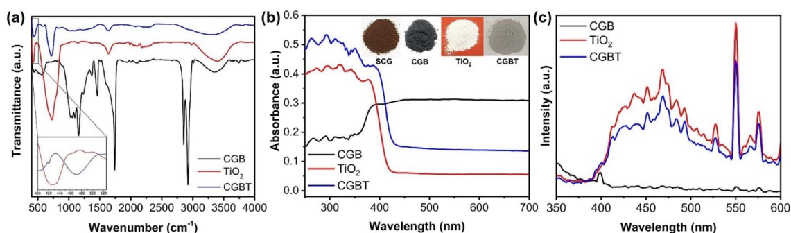
Fig. 3 (a) FT-IR spectra, (b) UV-vis DRS analysis (inset: picture of powder form of spent-coffee grounds (SCG), coffee-grounds biochar (CGB), TiO 2 , and coffee-ground biochar-supported TiO 2 nanocomposites (CGBT)), and (c) photoluminescence spectra of the synthesized materials.
