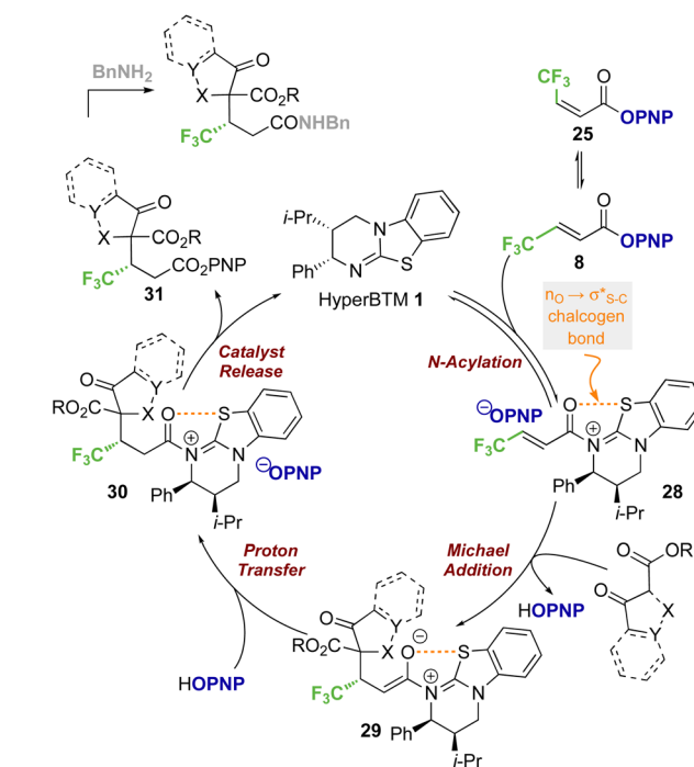
Scheme 7 Proposed simplified catalytic cycle.
