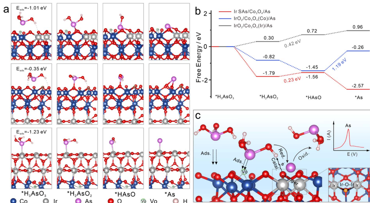
Fig. 4 Reduction reaction pathway analyses of \text{As(III)} on different catalysts. (a) Adsorption and stepwise reduction configurations of \text{H}_3\text{AsO}_3 on Ir SAs/ \text{Co}_3\text{O}_4 , \text{IrO}_2/\text{Co}_3\text{O}_4(\text{Co}) , and \text{IrO}_2/\text{Co}_3\text{O}_4(\text{Ir}) . (b) Relative energy of reduction intermediates of \text{H}_3\text{AsO}_3 on Ir SAs/ \text{Co}_3\text{O}_4 , \text{IrO}_2/\text{Co}_3\text{O}_4(\text{Co}) , and \text{IrO}_2/\text{Co}_3\text{O}_4(\text{Ir}) . (c) Proposed catalytic process of enhanced SWASV signals toward \text{As(III)} with Ir SAs/ \text{Co}_3\text{O}_4 .
