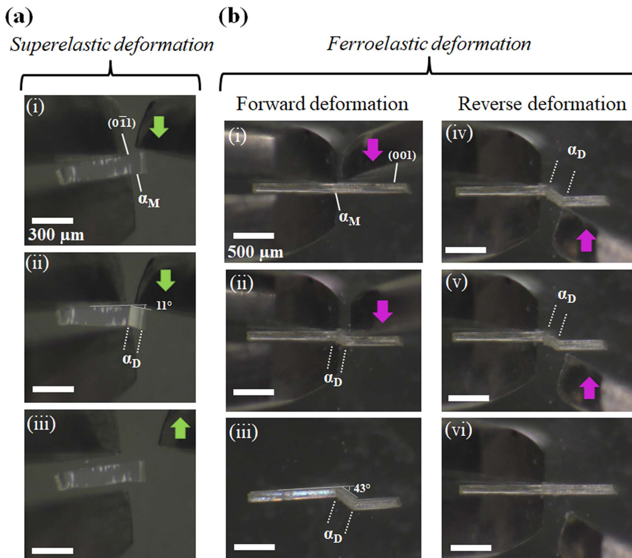
Fig. 2 Microscope observation with tweezers at room temperature: (a) superelastic deformation of cocystal 1 and (b) ferroelastic deformation of cocystal 2.
