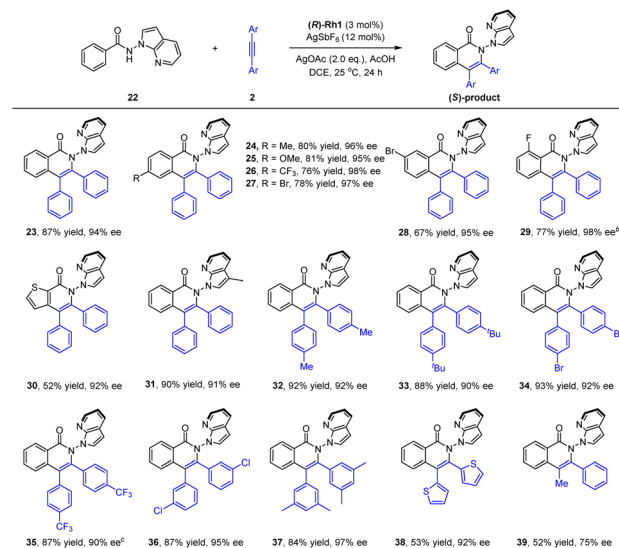
Scheme 3 Scope of N -azaindolyl benzamides as substrates for the synthesis of N - N atropisomers. (a) Reaction conditions: 1 (0.1 mmol), 2 (0.1 mmol), ( R )-Rh1 (3 mol%), AgSbF 6 (12 mol%), AgOAc (2.0 equiv.), AcOH (1.0 equiv.) in DCE (1 mL), 24 h, isolated yield. The ee was determined by HPLC using a chiral stationary phase. (b) 50 °C. (c) 25 °C, 60 h.
