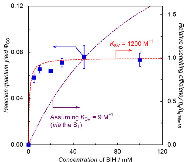
Fig. 11 Plot of the \Phi_{CO} versus the initial concentration of BIH in the photocatalytic \text{CO}_2 reduction (Xe lamp, 420 nm, 3.6 \times 10^{-8} einstein per s) using DMA–TEOA (4 : 1 v/v) solutions containing ZnP-5Bpy=Re Br (0.05 mM). The quenching efficiency relative to \eta_q at [BIH] = 50 mM was calculated using \eta_q = [\text{BIH}]K_{SV}/(1 + [\text{BIH}]K_{SV}) .
