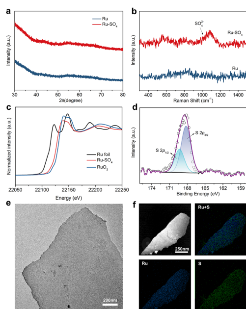
Fig. 1 (a) X-ray diffraction patterns of Ru and \text{Ru-SO}_4 . (b) Raman spectra of Ru and \text{Ru-SO}_4 . (c) Ru K-edge XANES of Ru foil, \text{Ru-SO}_4 and \text{RuO}_2 . (d) XPS spectra of S 2p for \text{Ru-SO}_4 . (e) Typical TEM image and (f) EDX mapping images for \text{Ru-SO}_4 .
