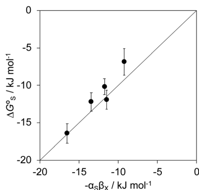
Fig. 13 Experimentally measured stabilisation of complex A in water due to resolution of the guest substituent X ( \Delta G^\circ_S ) compared with the calculated free energy change due formation of a H-bond between X and water ( -\alpha_S\beta_X ). The line corresponds to y = x .
