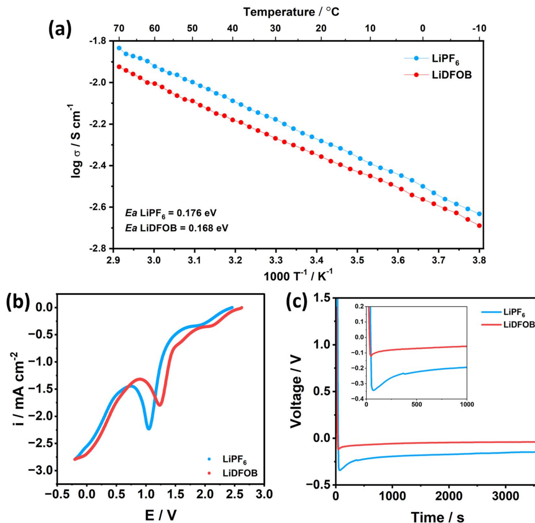
Fig. 2 (a) Arrhenius plot of 1 M \text{LiPF}_6 in EC : DEC (1 : 1, v/v) and 1 M \text{LiDFOB} in EC : DEC (1 : 1, v/v) electrolyte obtained with electrolyte conductivity measurement from 70^{\circ}\text{C} to -10^{\circ}\text{C} . The electrolyte conductivity was measured from -10 to 70^{\circ}\text{C} . (b) LSV scan of \text{Li}||\text{Cu} half cell with 1 M \text{LiPF}_6 and 1 M \text{LiDFOB} in EC : DEC (1 : 1, v/v) electrolyte with a scan rate of 0.1 \text{ V s}^{-1} . (c) Li plating overpotential at first discharge of \text{Li}||\text{Cu} half cell with 1 M \text{LiPF}_6 and 1 M \text{LiDFOB} in EC : DEC (1 : 1, v/v) electrolyte at a current density of 1 \text{ mA cm}^{-2} .
