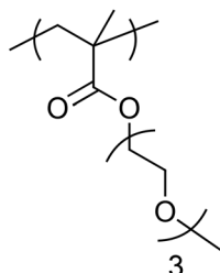
Poly[methoxy tri(ethylene glycol) methacrylate] (polymTEGMA, thermoresponsive, 49 \leq CP \leq 63 \text{ }^\circ\text{C} 17 )
