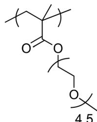
Poly[methoxy oligo(ethylene glycol) methacrylate with average M_n 300 \text{ g mol}^{-1} ] (polymOEGMA300, thermoresponsive, 71 \leq CP \leq 76 \text{ }^\circ\text{C} 17 )
