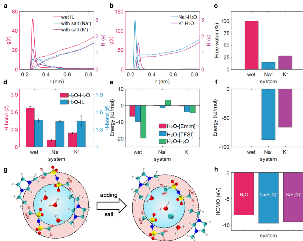
Fig. 1 Microscopic understanding of the salt effect on water in RTILs. (a) The RDF (left) and coordination number (right) of the mass-center of water with water in wet [\text{Emim}][\text{TFSI}] and salt-in-wet [\text{Emim}][\text{TFSI}] . (b) The RDF (left) and coordination number (right) of the mass-center of water with alkali ion salt-in-wet [\text{Emim}][\text{TFSI}] . (c) Proportion of free water in wet [\text{Emim}][\text{TFSI}] and salt-in-wet [\text{Emim}][\text{TFSI}] . (d) Hydrogen bond between water molecules (left) and water and ILs (right). (e) Interaction energy between water and [\text{Emim}]^+ (red), [\text{TFSI}]^- (blue), and water (green). (f) Interaction energy between alkali ions and water molecules. (g) Schematic of the solvation structure of water-in-wet [\text{Emim}][\text{TFSI}] and salt-in-wet [\text{Emim}][\text{TFSI}] . (h) HOMO energy levels of \text{H}_2\text{O} and \text{M}(\text{H}_2\text{O})^+ .
