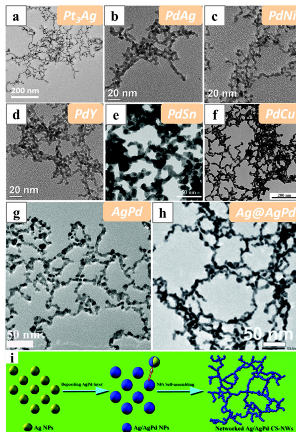
Fig. 15 TEM images of (a) Pt 3 Ag, (b) PdAg, (c) PdNi, (d) PdY, (e) PdSn, (f) PdCu, (g) AgPd and (h) Ag@AgPd nanowires synthesized with PVP as the structure-directing reagent in aqueous solutions. (i) Schematics illustrating the oriented attachment of Ag@AgPd nanoparticles into networked Ag@AgPd nanowires. Reprinted with permission from ref. 127–129, 131, 133 and 134. Copyright 2020 from Springer Nature, 2018 and 2021 from the Royal Society of Chemistry, 2017 from Elsevier.
