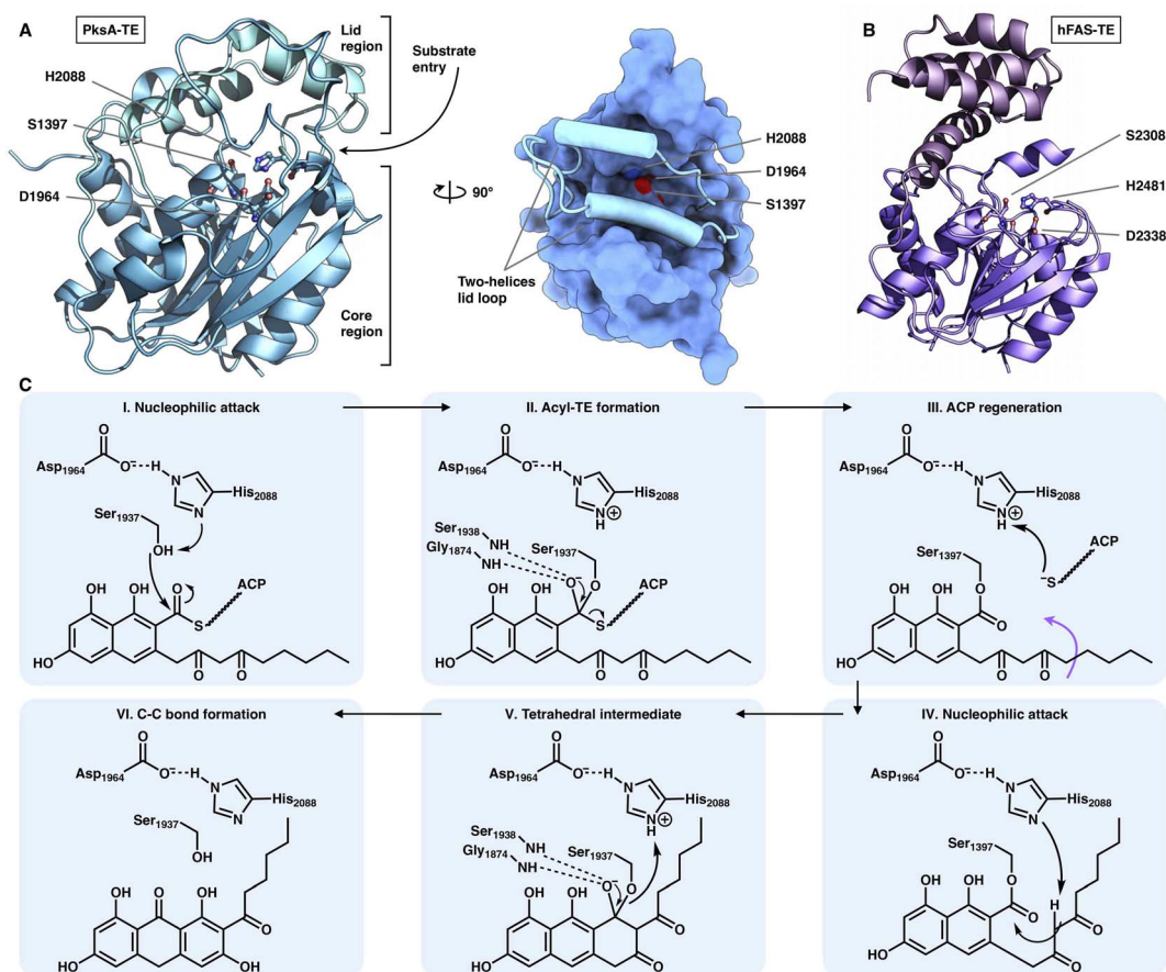
Fig. 17 Structures of the C-terminus-fused TEs. (A) TE structure of NR-iPKS PksA shown in both cartoon and surface representations, PDB: 3ILS. The S1397-D1964-H2088 catalytic triad is labeled. (B) hFAS TE domain, PDB: 1XKT. (C) Proposed catalytic mechanism of NR-iPKS PksA TE.
