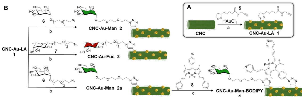
Scheme 1 A. Synthesis of CNC-Au-LA 1 . B. Synthesis of CNC-Au-Man 2 , CNC-Au-Fuc 3 , and CNC-Au-Man-BODIPY 4 . Reaction conditions: (a) NaBH 4 , MeOH : H 2 O (9 : 1), rt, 2 h; (b) CuSO 4 , sodium ascorbate, H 2 O, rt, 12 h; (c) CuSO 4 , sodium ascorbate, DMF, rt, 12 h.
