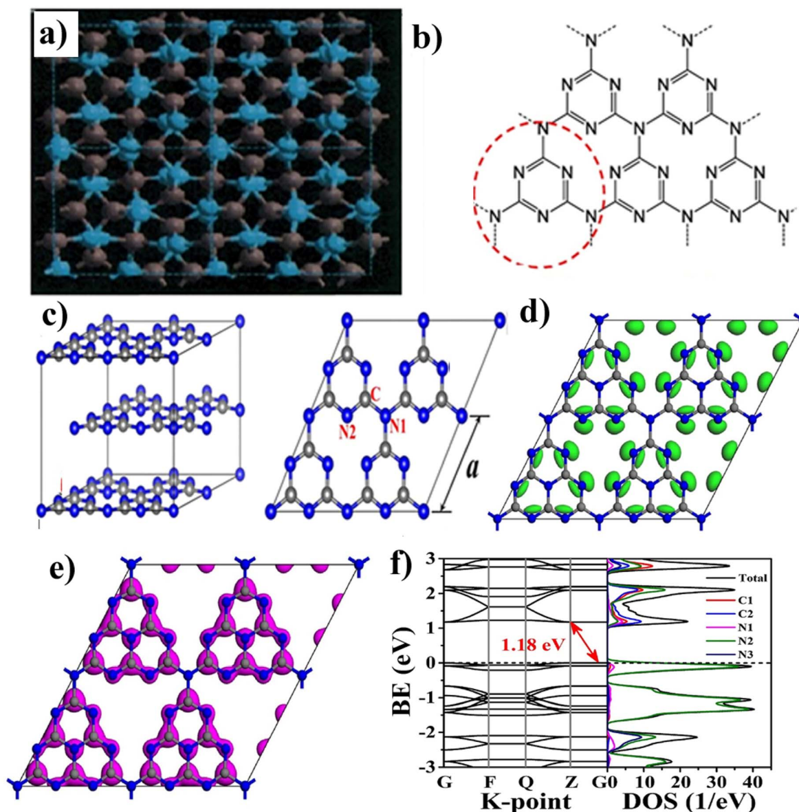
Fig. 4 (a) Cubic- \text{C}_3\text{N}_4 structures down the [001] axis, showing grey spheres (C atoms) and blue (N atoms), (b) s -triazine, heptazine structures of g - \text{C}_3\text{N}_4 (reproduced with permission from ref. 66 Copyright 2017, Springer Nature). (c) Geometric structures of g - \text{C}_3\text{N}_4 bulk and g - \text{C}_3\text{N}_4 monolayer, DFT structure (reproduced with permission from ref. 75 Copyright 2019, Wiley Online Library). (d) Calculated HOMO, (e) LUMO, (f) band structure and corresponding DOS of monolayer g - \text{C}_3\text{N}_4 (G, F, Q, and Z are high symmetry points in the reciprocal space) (reproduced with permission from ref. 76 Copyright 2017, Elsevier).
