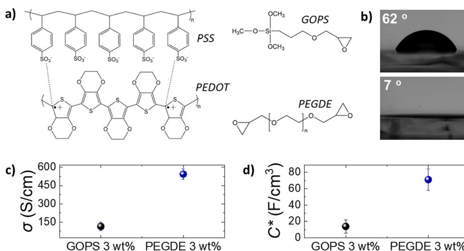
Fig. 1 (a) The chemical structures of the conducting polymer PEDOT:PSS and the crosslinkers (3-(glycidyloxypropyl)trimethoxysilane (GOPS) and poly(ethylene glycol)diglycidyl ether. (b) Digital pictures of the water contact angle on top of a PEDOT:PSS film crosslinked with GOPS 3 wt% (top) and with PEGDE 3 wt% (bottom). (c) Electrical conductivity ( \sigma ) and (d) volumetric capacitance ( C^* ) of PEDOT:PSS films crosslinked with GOPS 3 wt% and PEGDE 3 wt%. Error bars represent the standard deviation of six replicates for each condition (mean \pm SD, n = 6 ).
