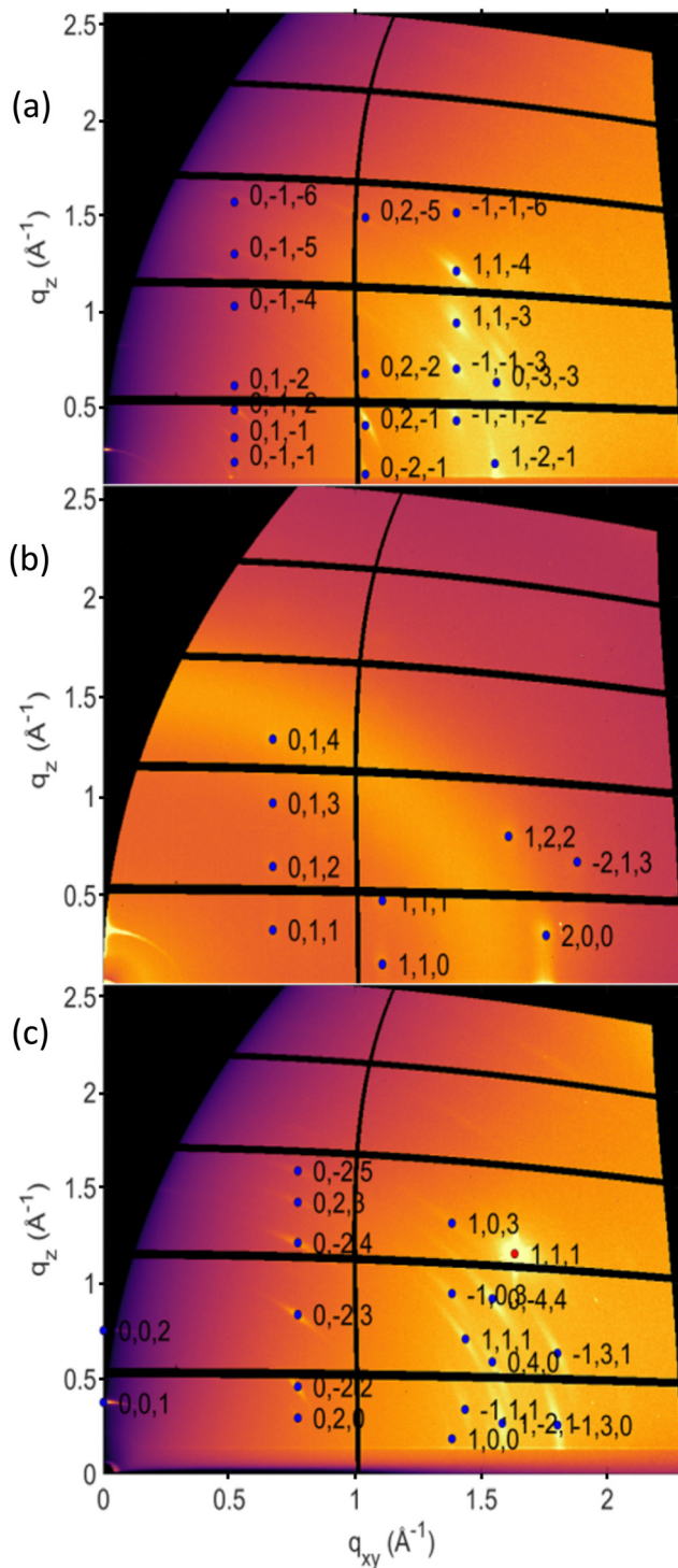
Fig. 3 Grazing incidence X-ray diffraction images recorded on three thin-film phases of OEG- BTBT: (a) Form IV, (b) Form V, and (c) Form VI. Indexing of the Bragg peaks (blue points) reveals the corresponding crystallographic lattices; a single diffraction peak of the silicon substrate is observed (red point).
