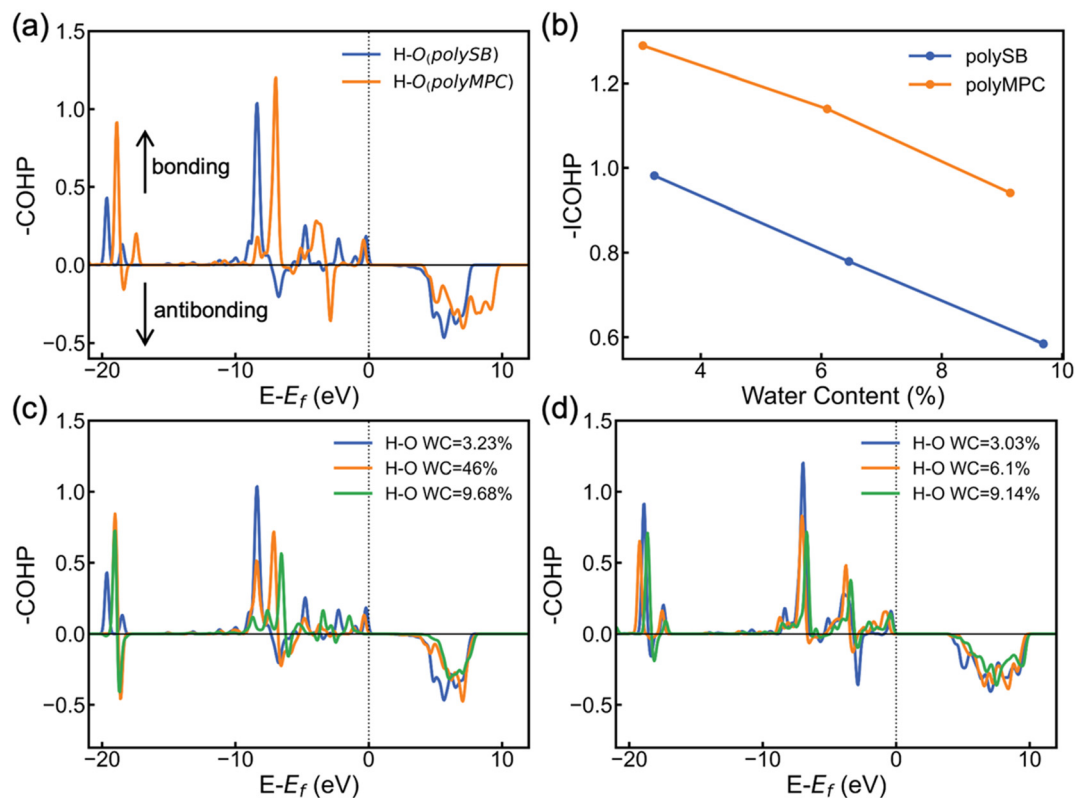
Fig. 5 (a) Crystal orbital Hamilton population (COHP) of the bond between hydrogen atom of the adsorbed H_2O and the nearest oxygen of polySB and polyMPC at WC = 3.23% and 3.03%, respectively. (b) Integrated COHP (ICOHP) vs. water content, calculated COHP for the bond between hydrogen atom of adsorbed H_2O and nearest oxygen atom of the polySB (c) and polyMPC (d) at different WC.
