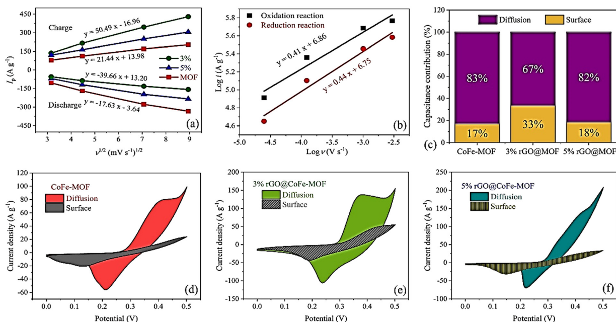
Fig. 18 (a) The curves of the peak current versus the square root of sweep rate (Randles–Sevcik plot). (b) The plots of log i versus log \nu . (c) Capacitance contribution for three electrodes, the capacitive contribution of CV curves at 10 mV s -1 for (d) CoFe-MOF, (e) 3% rGO@CoFe-MOF, and (f) 5% rGO@CoFe-MOF. Reproduced from ref. 173 with permission from Elsevier Ltd, Copyright 2023.
