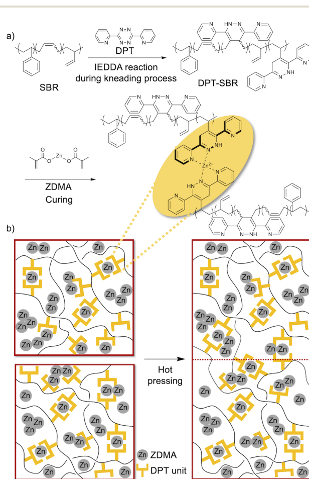
Fig. 1 Conceptual outline of this study: (a) preparation of DPT-modified SBRs by IEDDA reactions during the kneading process, followed by the formation of DPT–ZDMA cross-linkages and (b) schematic description of the adhesion process via rearrangement of the DPT–ZDMA cross-linkages.
