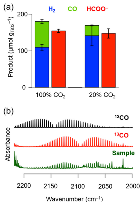
Fig. 2 (a) \text{H}_2 , CO and formate (blue, green and red, respectively) formation after 24 h of photocatalysis with \text{TiO}_2|\text{CotpyP} . (b) Transmission IR spectra with ^{13}\text{CO}_2 isotopic labelling of the headspace after 24 h of photocatalysis (sample, green curve), including ^{12}\text{CO} (black) and ^{13}\text{CO} (red) as reference. Reaction conditions: 5 mg \text{TiO}_2 (P25); 50 nmol \text{CotpyP} ; 3 mL 2 : 1 MeCN : pre-treated reaction solution (cellulose fraction pre-treated with cellulase); 25 °C, 100 \text{mW cm}^{-2} , AM 1.5G. (a) 20 vol% \text{CO}_2 was balanced with \text{N}_2 ; (b) sample (green) was purged with 100% ^{13}\text{CO}_2 . Experiments in (a) were performed in triplicates.
