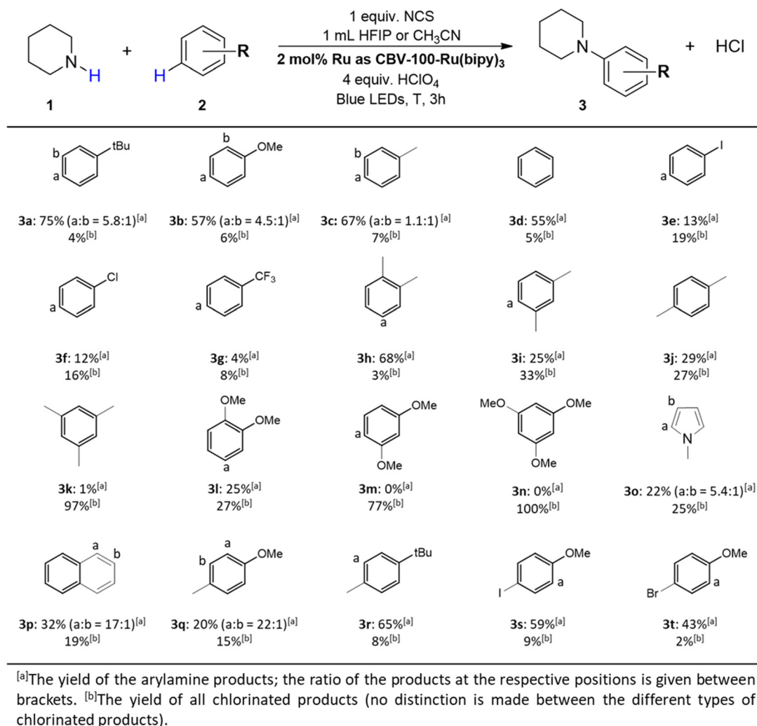
Fig. 7 Substrate scope of different arene substrates. Reaction conditions: 1 (0.1 mmol), NCS (1 equiv.), 1 mL HFIP or CH 3 CN were mixed together and stirred for 30 minutes, afterwards 2 (18 equiv.), CBV-100-Ru(bipy) 3 (2 mol% Ru), HClO 4 (4 equiv.) were added and the suspension was exposed to blue lights (455–470 nm, 40 W), for 3 h at 0 °C, –20 °C or –40 °C.
