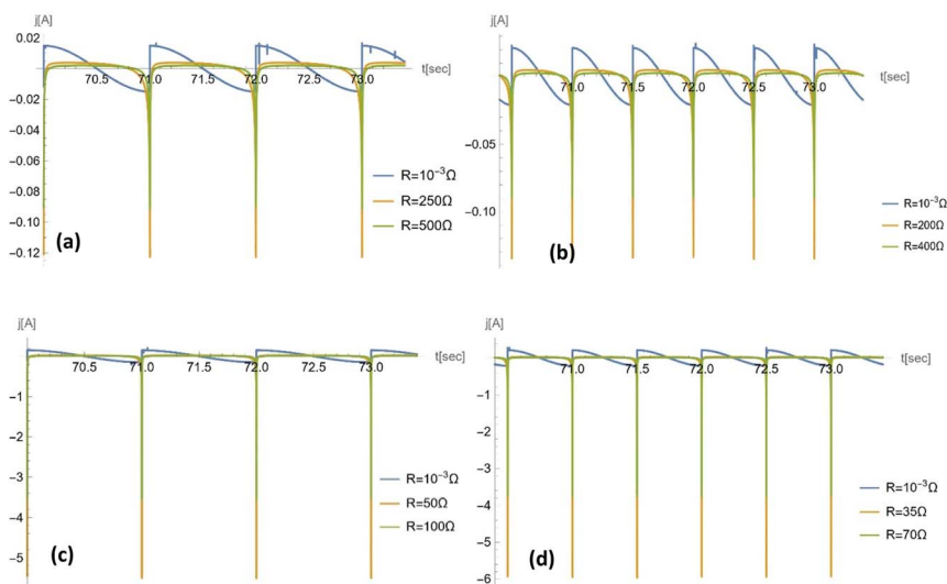
Fig. 9 Temporal profile of the electrical current for a porous electrode. For a pore size of r_p = 10^{-5} \text{ m} , the frequency used is (a) \omega = 2\pi \text{ s}^{-1} and (b) \omega = 4\pi \text{ s}^{-1} ; for a pore size of r_p = 10^{-7} \text{ m} , the frequency used is (c) \omega = 2\pi \text{ s}^{-1} and (d) \omega = 4\pi \text{ s}^{-1} . For each plot, 3 different loads were chosen on the basis of: (1) near-zero value, which shows a temporal profile consistent with the literature with consideration of no/negligible load; 23 (2) resistance at which the power reaches maximum; and (3) resistance larger than that corresponding to the maximum power. Other parameters used are: V_{\text{ref}} = 1.5 \text{ V} , \bar{C} = 5 \times 10^{-2} \text{ F m}^{-2} ; S_T = 0.002 \text{ m}^2 ; \varepsilon = 0.5 ; \theta_w = 131.18^\circ ; \eta = 6.3 \times 10^{-2} \text{ Pa s}^{-1} ; and \gamma = 2.27 \times 10^{-2} \text{ N m}^{-1} .
