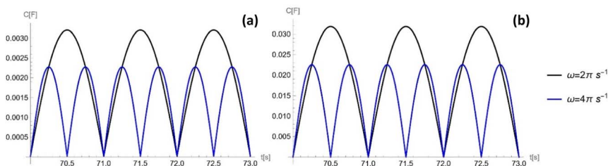
Fig. 8 Capacitance generated over time at the frequency of 2\pi \text{ s}^{-1} (black) and 4\pi \text{ s}^{-1} (blue) for a porous electrode. The pore size r is 10^{-5} \text{ m} for (a) and 10^{-7} \text{ m} for (b). Parameters used are: \bar{C} = 5 \times 10^{-2} \text{ F m}^{-2} ; S_T = 0.002 \text{ m}^2 ; \varepsilon = 0.5 ; \theta_w = 131.18^\circ ; V_{\text{ref}} = 1.5 \text{ V} ; \eta = 6.3 \times 10^{-2} \text{ Pa s}^{-1} ; and \gamma = 2.27 \times 10^{-2} \text{ N m}^{-1} .
