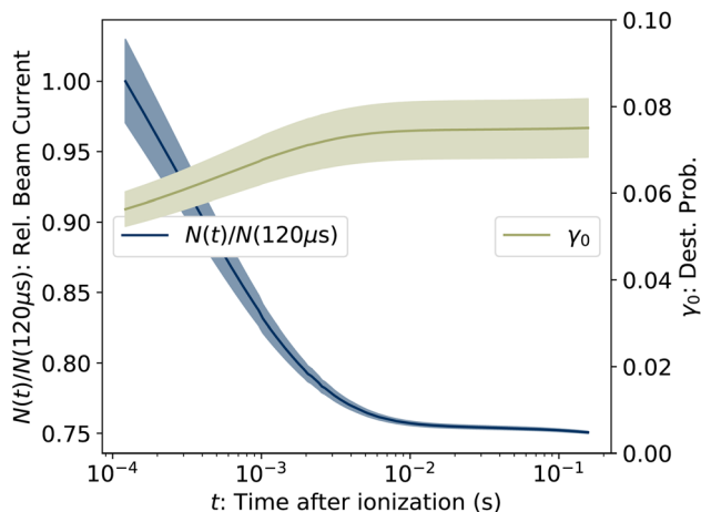
Fig. 3 (Left axis) Number of ions stored in the measurement of R(t) , relative to the value at the first time point at t = 120\mu\text{s} . (Right axis) Ensemble averaged destruction probability \gamma_0 , determined from eqn (5). The shaded areas give the uncertainties.
