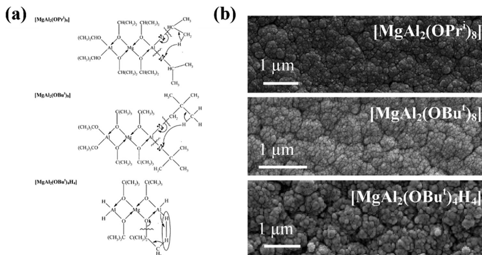
Fig. 16 (a) Proposed decomposition methods and (b) scanning electron microscopy surface images for precursors (top to bottom) [\text{MgAl}_2(\text{OPr})_6] , [\text{MgAl}_2(\text{OBu})_6] , [\text{MgAl}_2(\text{OBu})_4\text{H}_4] . Reproduced with permission from ref. 204 copyright 2004, American Chemical Society.
