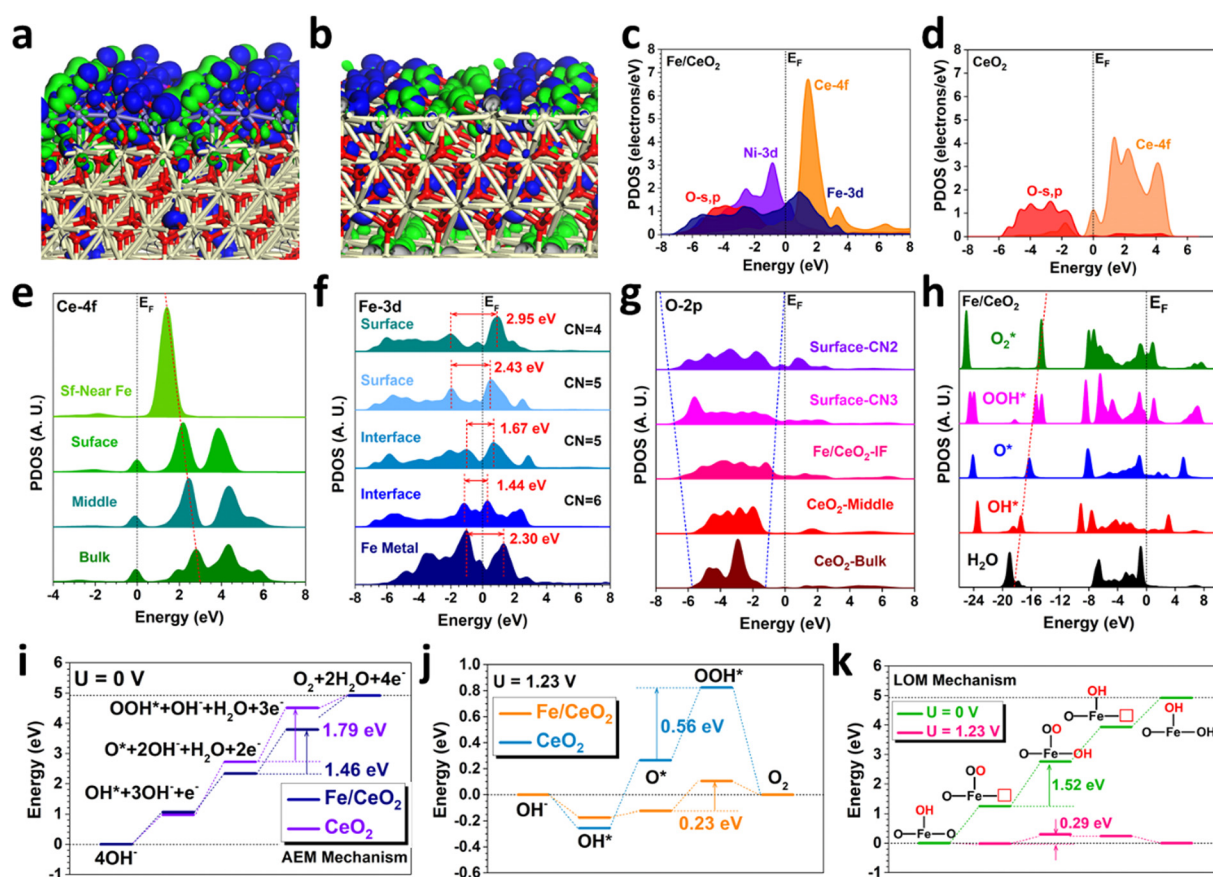
Fig. 4 DFT calculations. (a) The 3D contour plot of electronic distribution near the Fermi level of \text{Fe}/\text{CeO}_2 . (b) The 3D contour plot of electronic distribution near the Fermi level of \text{CeO}_2 . Yellow balls = Ce, Blue balls = Fe, Purple balls = Ni, and Red balls = O. Blue isosurface = bonding orbitals, and green isosurface = anti-bonding orbitals. (c) The PDOS of \text{Fe}/\text{CeO}_2 . (d) The PDOS of \text{CeO}_2 . (e) The site-dependent PDOS of Ce-4f in \text{Fe}/\text{CeO}_2 . (f) The site-dependent PDOS of Fe-3d in \text{Fe}/\text{CeO}_2 . (g) The site-dependent PDOS of O-2p in \text{Fe}/\text{CeO}_2 . (h) The PDOS of key adsorbates during the OER process in \text{Fe}/\text{CeO}_2 . (i) The reaction energy changes of the OER process on \text{Fe}/\text{CeO}_2 and \text{CeO}_2 under U = 0 \text{ V} through the AEM mechanism. (j) The reaction energy changes of the OER process on \text{Fe}/\text{CeO}_2 and \text{CeO}_2 under U = 1.23 \text{ V} through the AEM mechanism. (k) The reaction energy changes of \text{Fe}/\text{CeO}_2 through the LOM mechanism.
