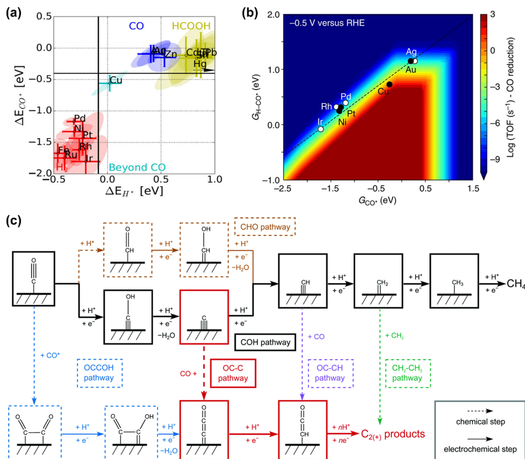
Fig. 2 (a) Metal classification for \text{CO}_2 electroreduction. Reproduced with permission. 23 Copyright 2017, Wiley. (b) Rate map at -0.5 \text{ V} versus reversible hydrogen electrode (RHE) for \text{CH}_4 formation over Cu. Reproduced with permission. 82 Copyright 2017, Nature. (c) Schematic diagram of reaction steps for \text{C}_{2+} over Cu. Reproduced with permission. 84 Copyright 2021, from RSC Publishing.
