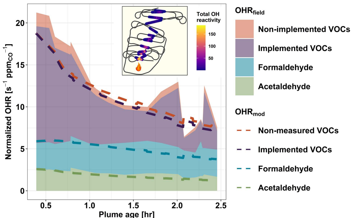
Fig. 5 Field and modeled normalized OHR ( \text{s}^{-1} \text{ppmCO}^{-1} ) for the Taylor Creek Fire sampled during WE-CAN with the inset plot showing the corresponding flight track shaded by the total OHR for each plume transect. Shaded regions represent the total calculated OHR from observations, while dashed lines are the model predicted OHR. Formaldehyde and acetaldehyde are shown separately as they are two of the largest contributors to the VOC OHR and important model diagnostics. The purple shading and dashed line represent VOCs measured in the field which are also included in the model. The red shading and dashed line is the combination of measured but not modeled plus modeled but not measured VOCs and show their combined impact is relatively insignificant.
